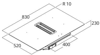
Standardmontering
